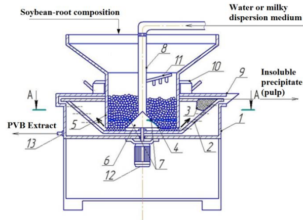
Figure 2: Diagram of the device for cooking SVB: 1 - body; 2 - perforated tapered rotor; 3 - filter; 4 - the base of the rotor; 5 - pipe; 6 - funnel element; 7 - stops; 8 - tube for the supply of the extractant; 9 - reflector visor; 10 - adjusting nut; 11 - metering lever.
