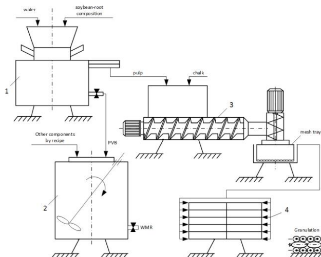
Figure 3: Constructive-technological scheme of the line for the preparation of WMR and granular additives
