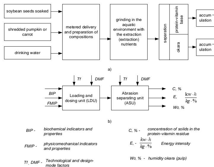
Figure 1: Technological (a) and structural-functional (b) process diagrams and devices for obtaining PVB for WMR
