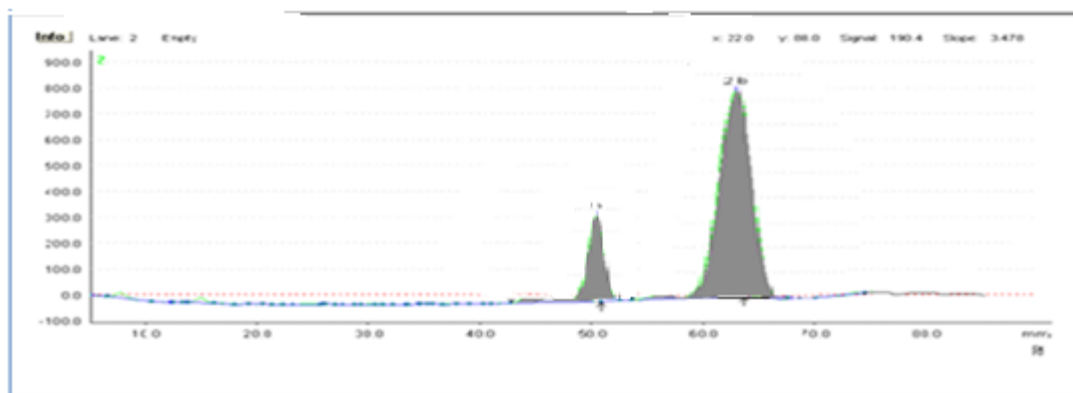
Fig 2: Typical HPTLC chromatogram 1) Diclofenac 2) Paracetamol
