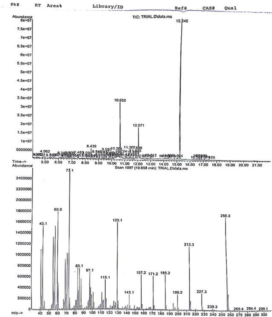
Figure – 1: GC- MS chromatogram of Calotropis gigantea
