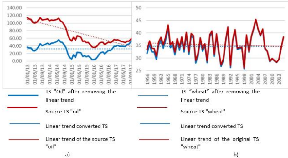
(a) TS "oil" from 21.12.12 to 21.12.17; (b) TS "wheat" from 1956 to 2015 Figure 1: Time series charts before and after removing a linear trend
