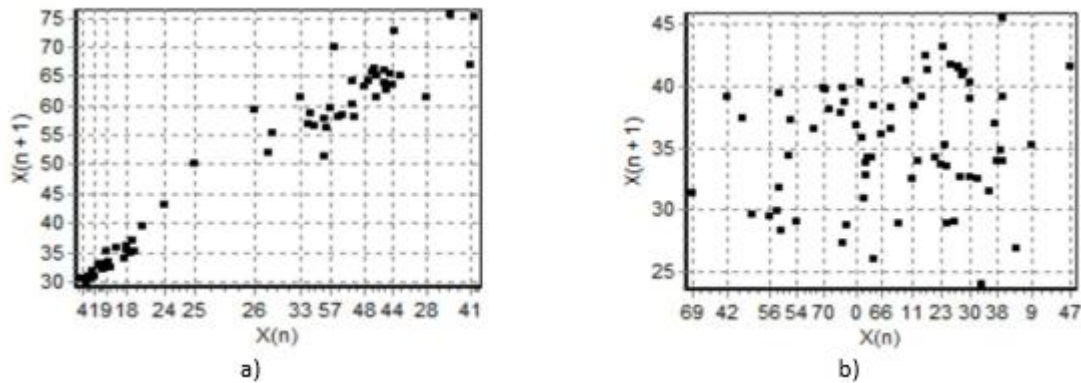
(a) TS "oil" from 21.12.12 to 21.12.17; (b) TS "wheat" from 1956 to 2015 Figure 2: Pseudo-phase time series spaces
