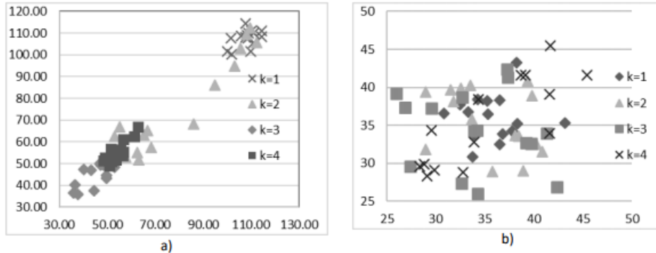
(a) TS "oil" from 21.12.12 to 21.12.17; (b) TS "wheat" from 1956 to 2015 Figure 3: Test results for a drift attractor:
