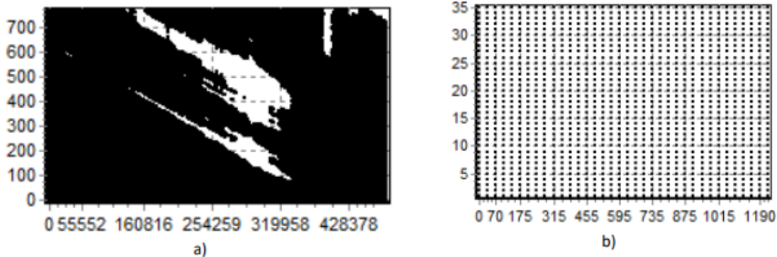
Figure 4: Gilmore test results for: (a) TS "oil" from 21.12.12 to 21.12.17; (b) TS "wheat" from 1956 to 2015
