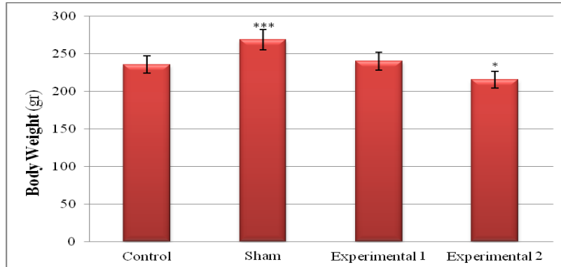
Fig 1: Comparing the weights of the various groups the 8th week study (***: P<0.001; *: P<0.05).
