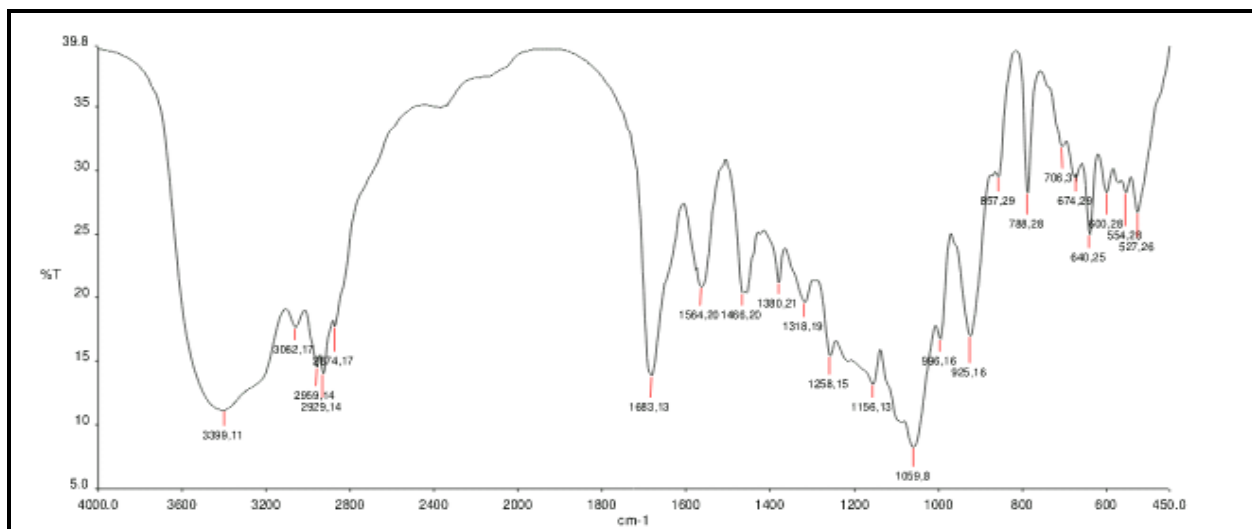
Fig. 5: FTIR Spectra of mixture of Clindamycin phosphate and HPMC-5
