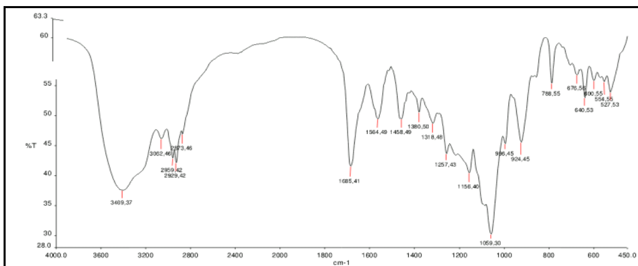
Fig. 6: FTIR Spectra of mixture of Clindamycin phosphate and HPMC-15
