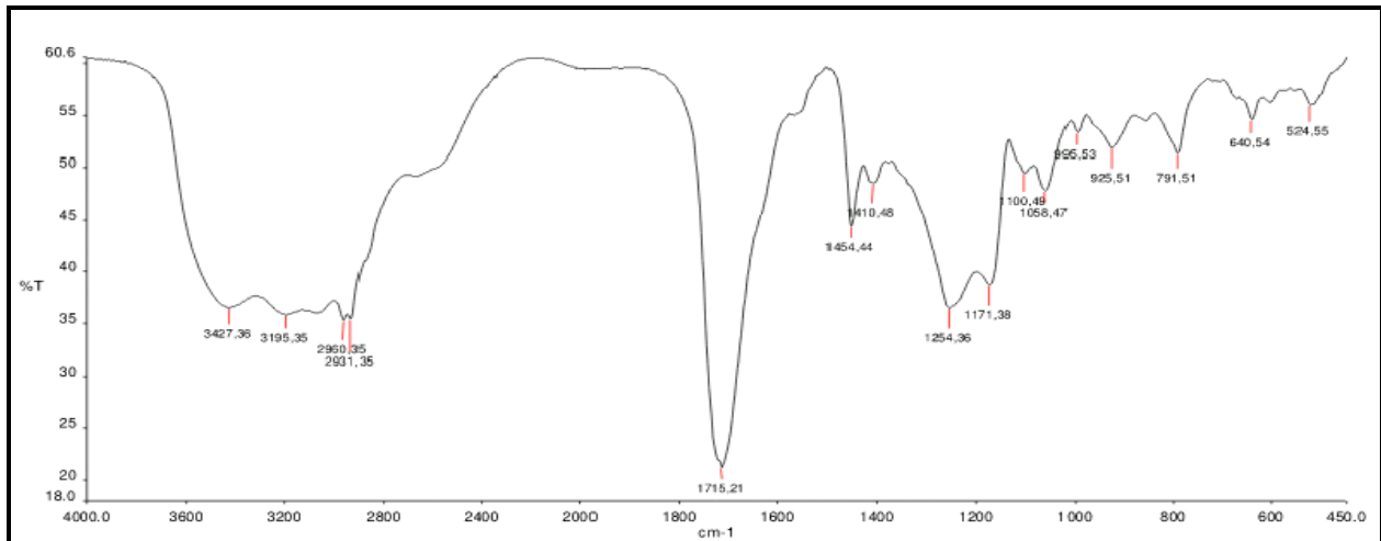
Fig. 3: FTIR Spectra of mixture of Clindamycin phosphate and Carbopol-934
