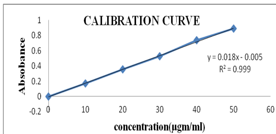
Fig 2: Calibration curve for Metformin Hydrochloride in pH 1.2HCl buffer.
