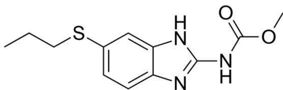
Figure 1 ALBENDAZOLE STRUCTURE
